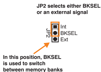
Figure 8. BUF08821EVM Jumper JP2 Set for BKSEL Switching
