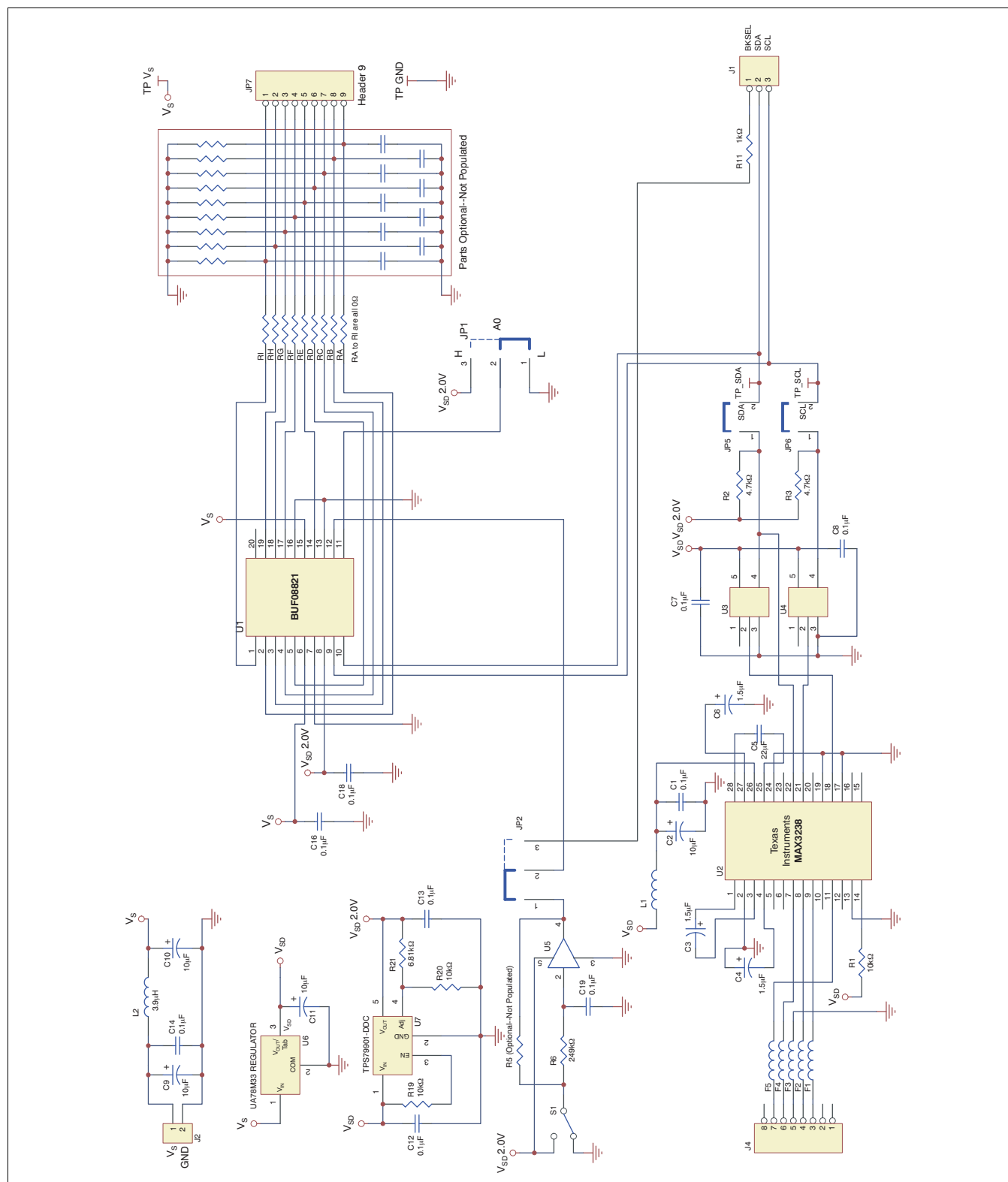
Figure 22. BUF08821EVM Schematic
